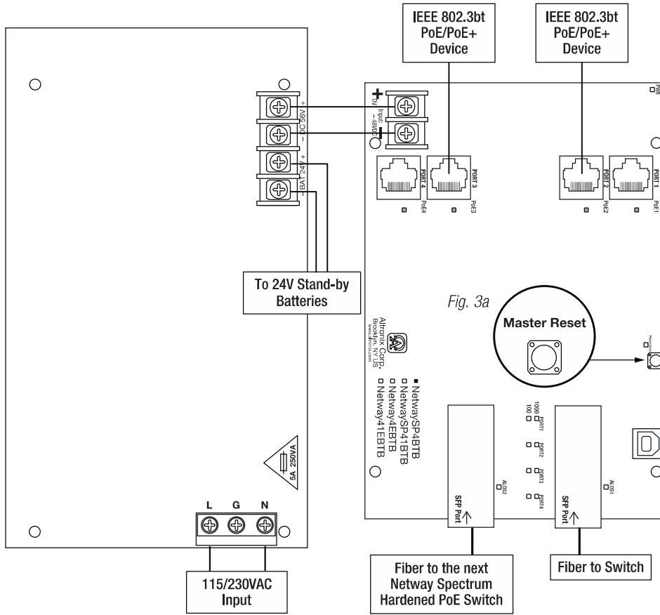
Fig. 3 - NetWaySP4BTX/NetWaySP4BTWP/NetWaySP4BTWPX/NetWaySP4BL – Typical Application with Factory Installed Power Supply
