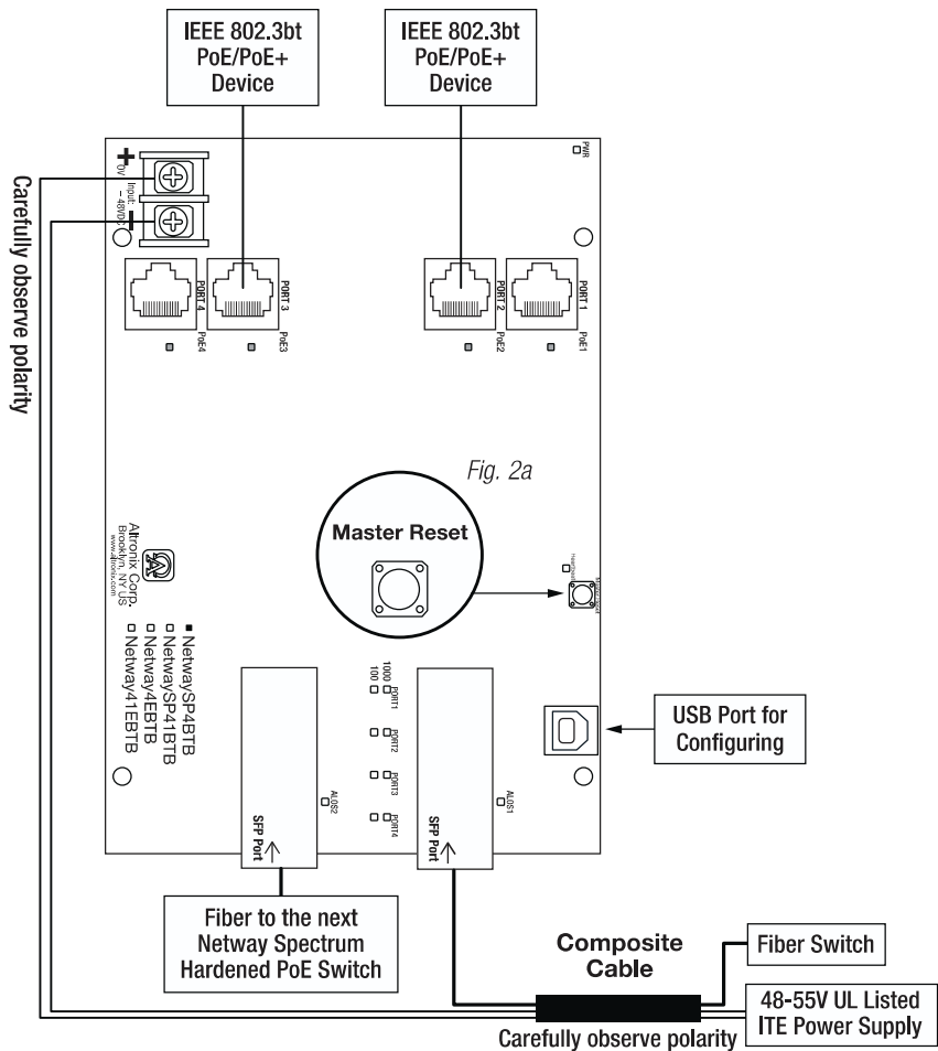
Fig. 2 - NetWaySP4BTB/NetWaySP4BTWPN – Typical Application with Composite Cable
