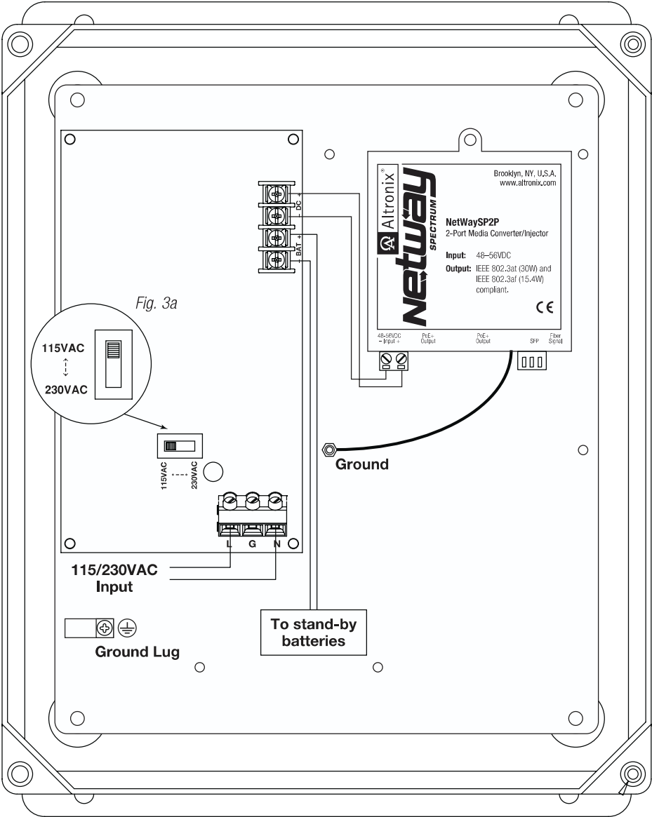
Fig. 3 - NetWaySP2PWP Configuration
