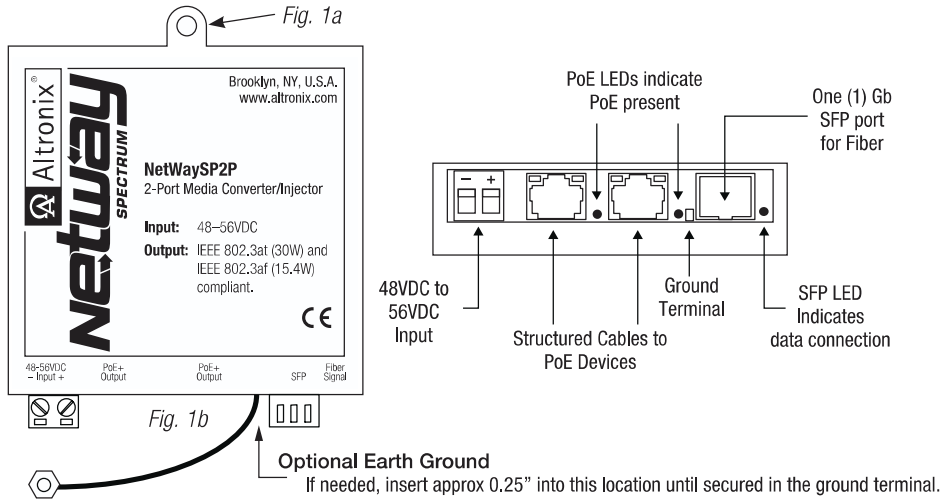
Fig. 1 - NetWaySP2P Configuration
