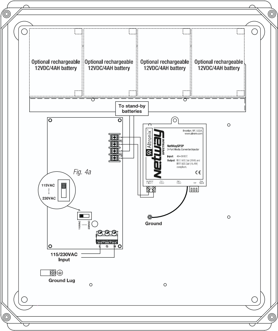
Fig. 4 - NetWaySP2PWPX Configuration
