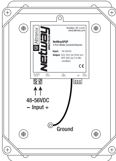
Fig. 2 - NetWaySP2PWP Configuration
