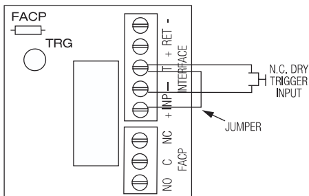
Fig. 14 Normally Closed: Non-Latching FACP trigger input:
