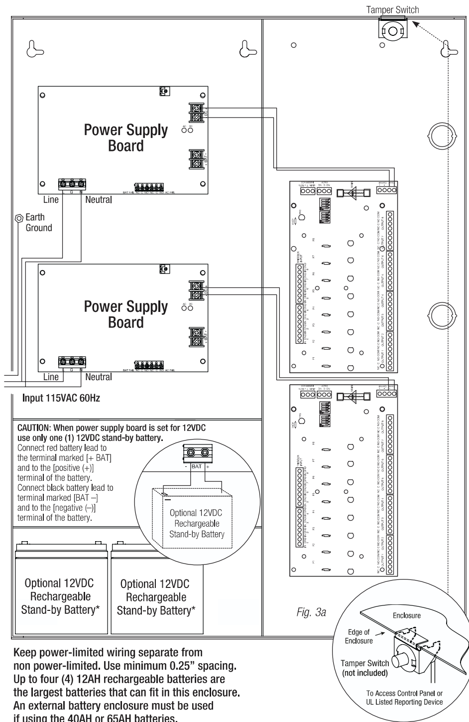
Fig. 3 - Maximal11D, Maximal33D, Maximal55D
