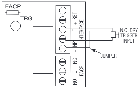
Fig. 14 Normally Closed: Non-Latching FACP trigger input:
