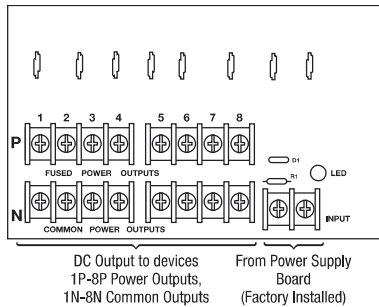
Fig. 3b - PD8ULCB Power Distribution Board Class 2 Power-Limited Outputs
