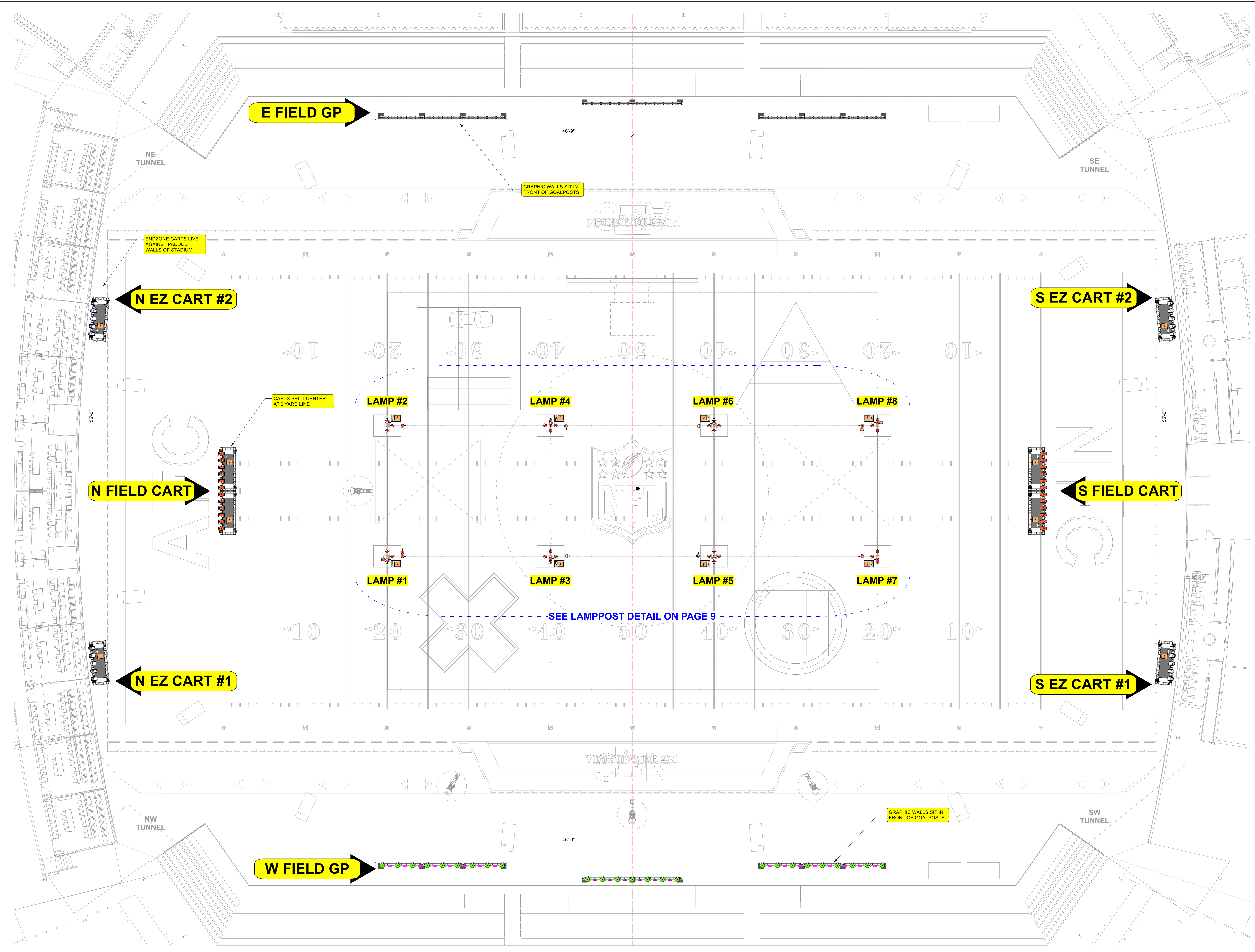
1 FIELD LEVEL LAYOUT Scale: 3/32" = 1'-0"
