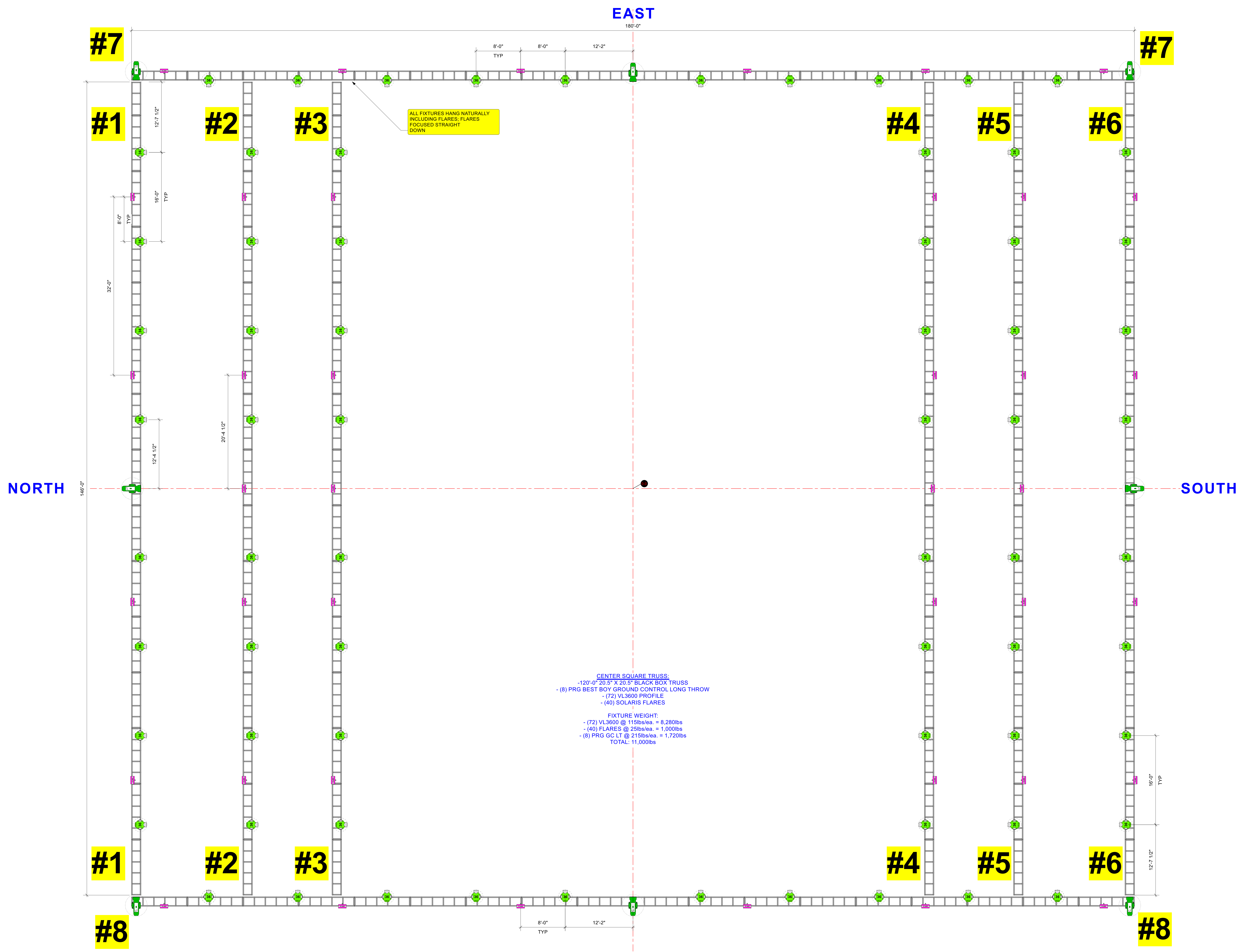
1 CENTER SQUARE TRUSS Scale: 3/16" = 1'-0"
