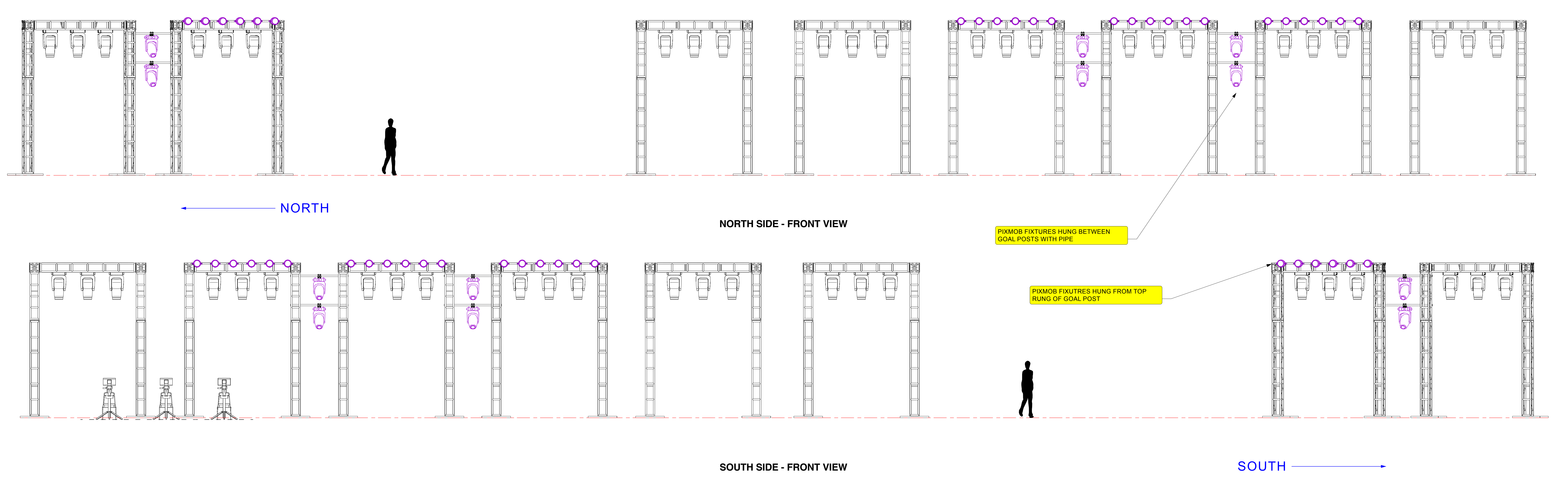
2 FOH GOALPOST DETAIL Scale: 1/4" = 1'-0"
