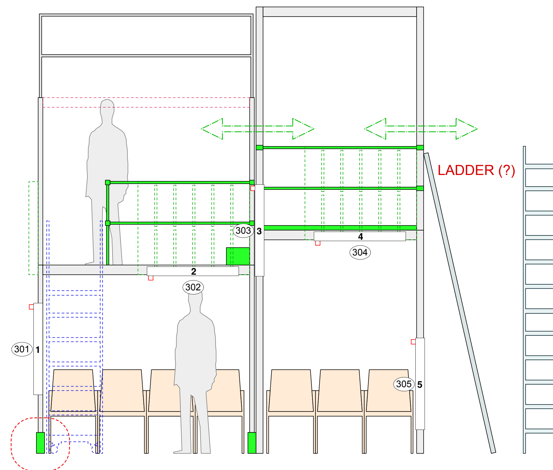
SR. SCAFFOLDING
