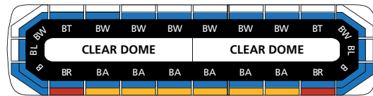
RLNT48-P2LC (without interface module, low hook mount)
