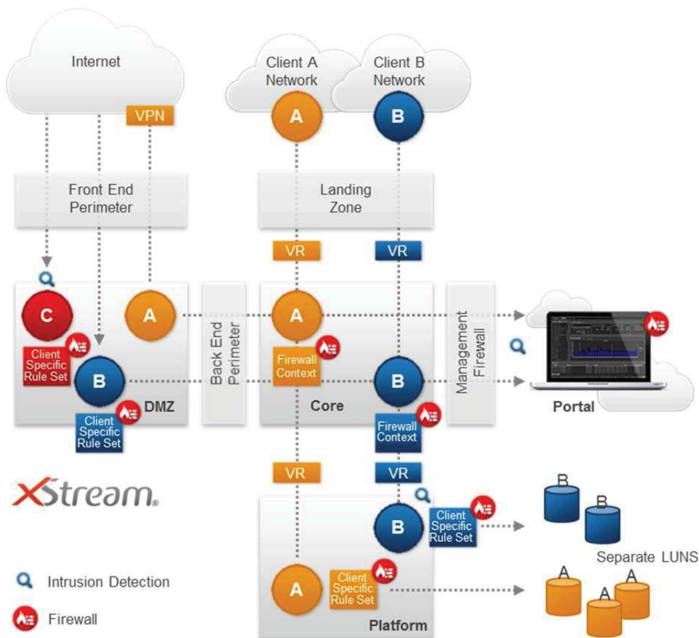
Figure 16. xStream Enterprise Architecture
