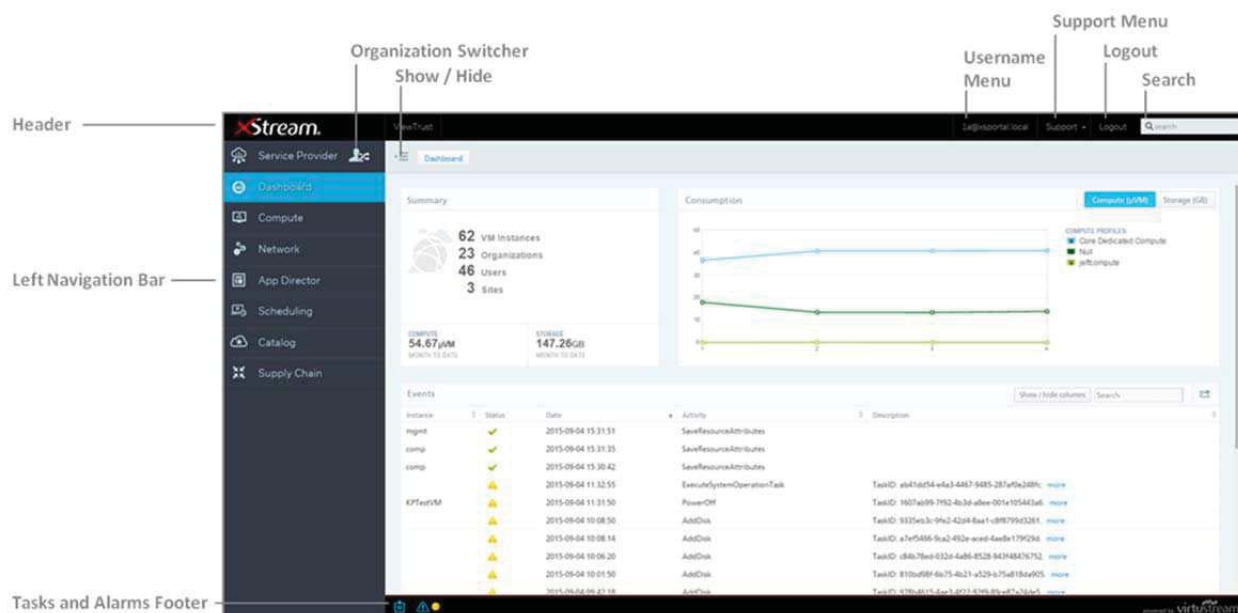
Figure 7. xStream Portal Sample View
