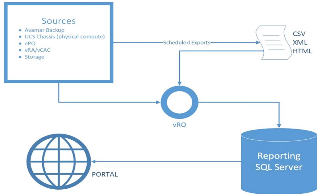
Figure 16. Report Workflow
