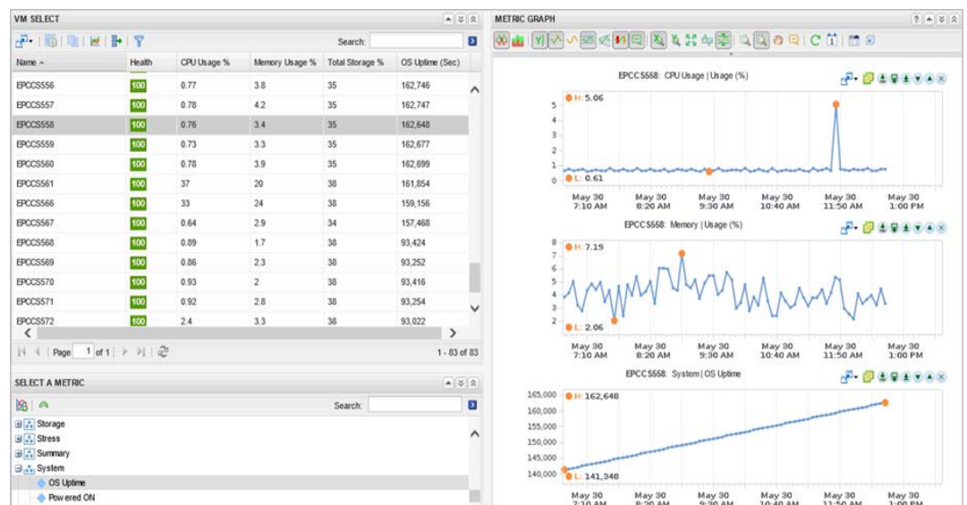
Figure 17. Performance Statistics
