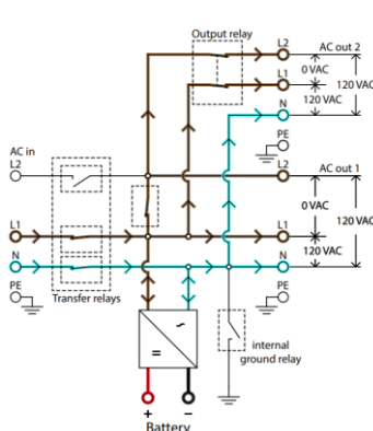
Vermogenstroom, 120 VAC-invoer
