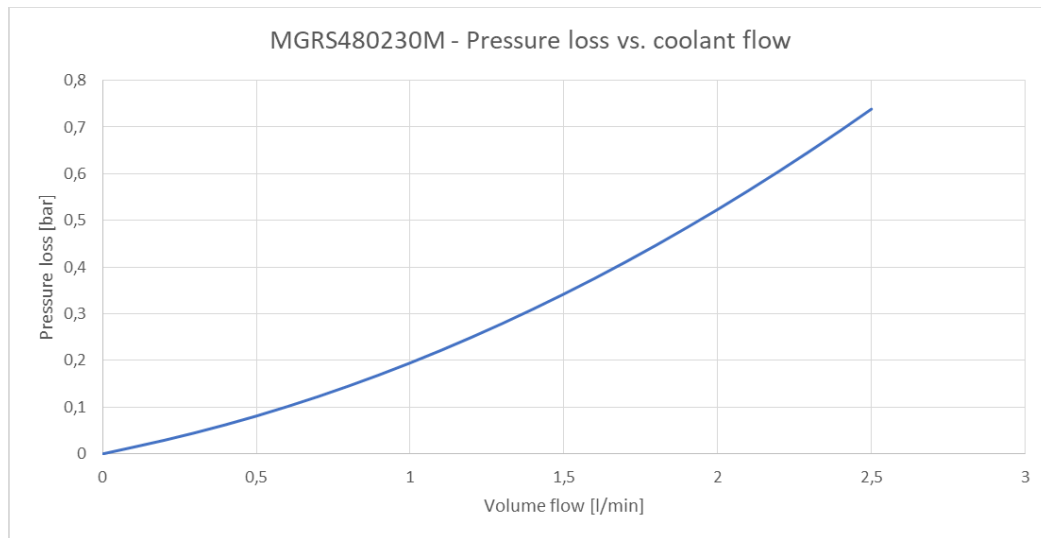
Figure 18 - Pressure loss versus cooling flow
