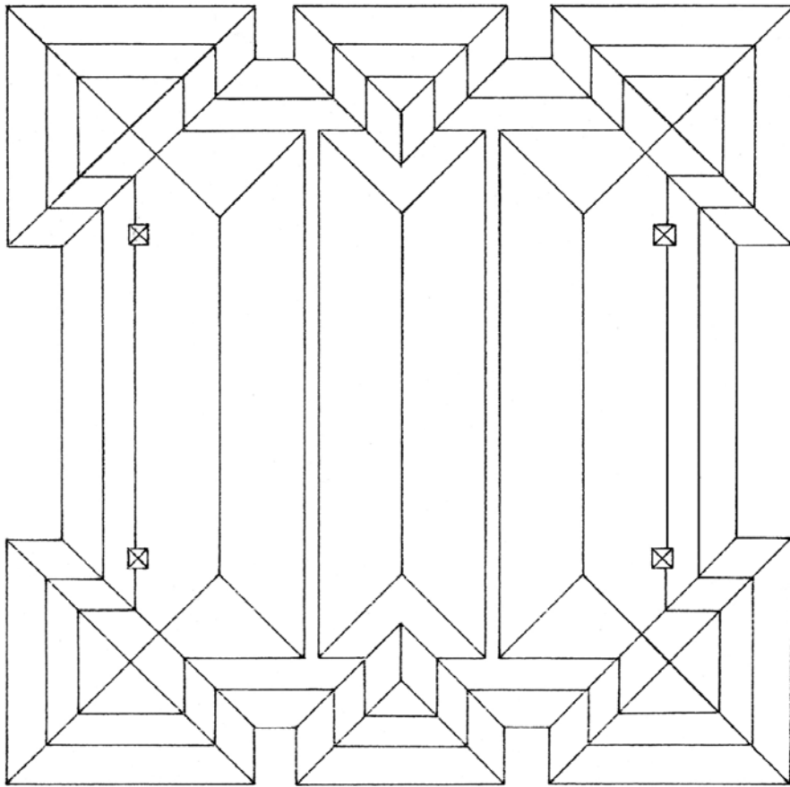
ROOF PLAN
