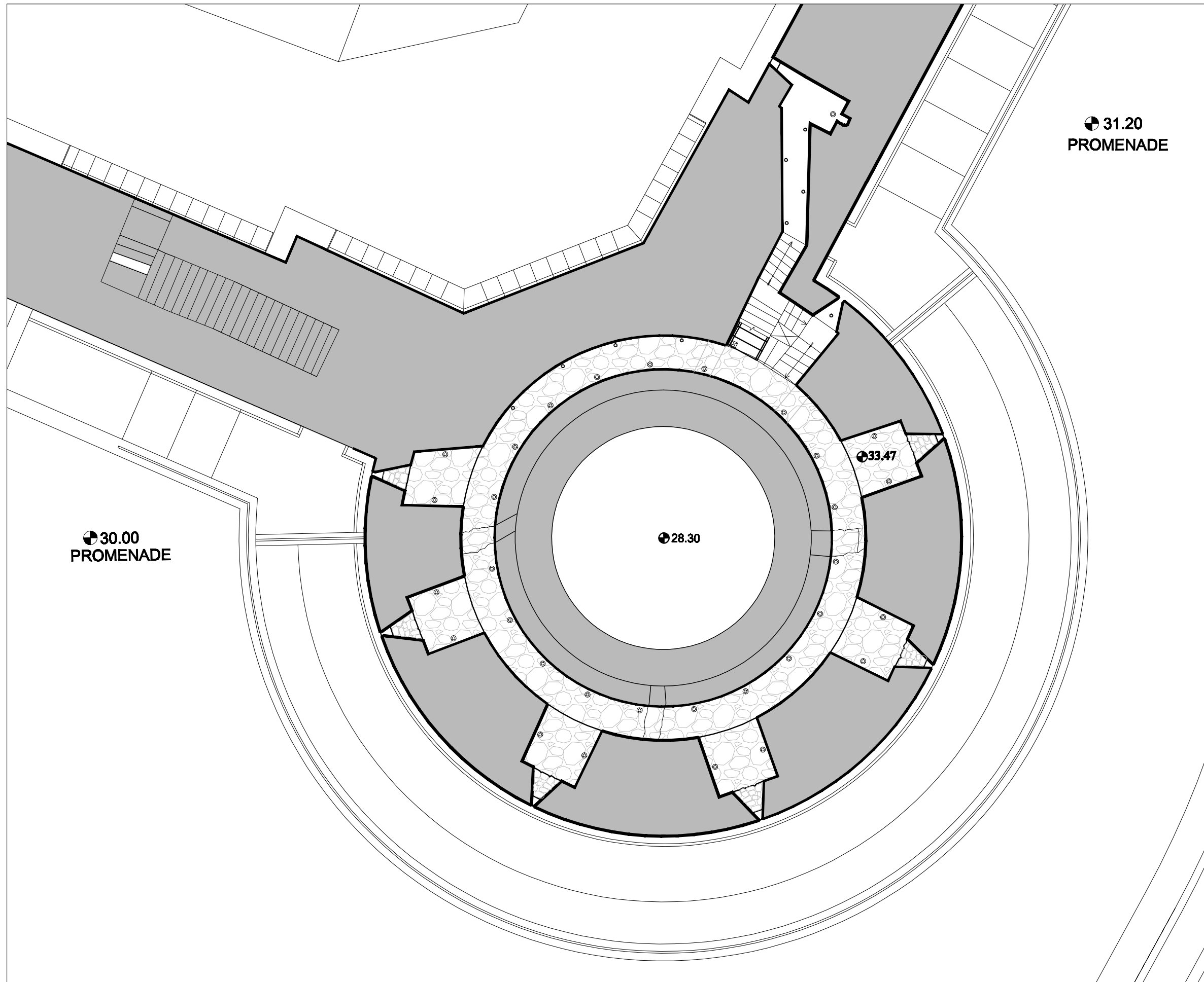
1 First floor plan ( after ) Tower 10
