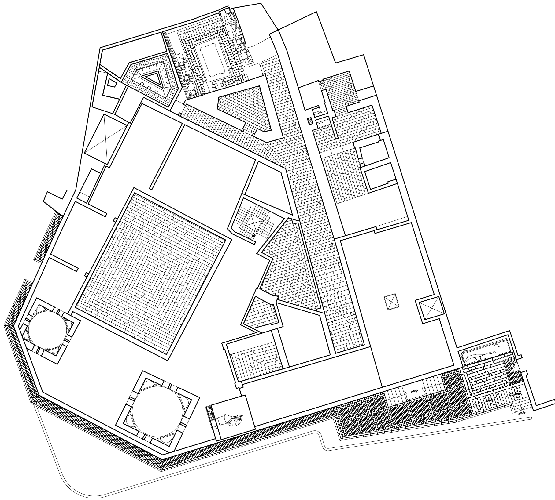
ROOF PLAN A-03
