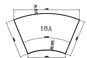
Bottom Plan Final Carved Stone NM18A plans 1:50
