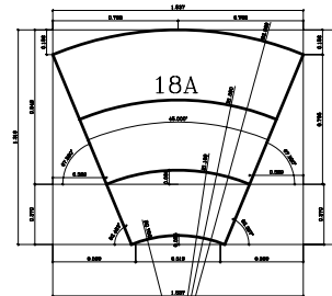
Ashler NM18A plan 1:50
