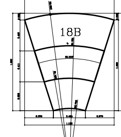
Ashler NM18B plan 1:50
