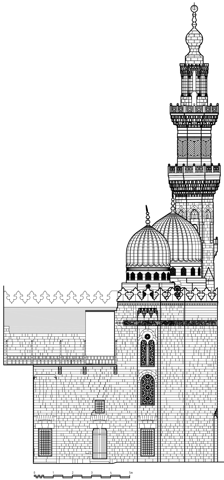
B 02 SOUTH WEST ELEVATION
