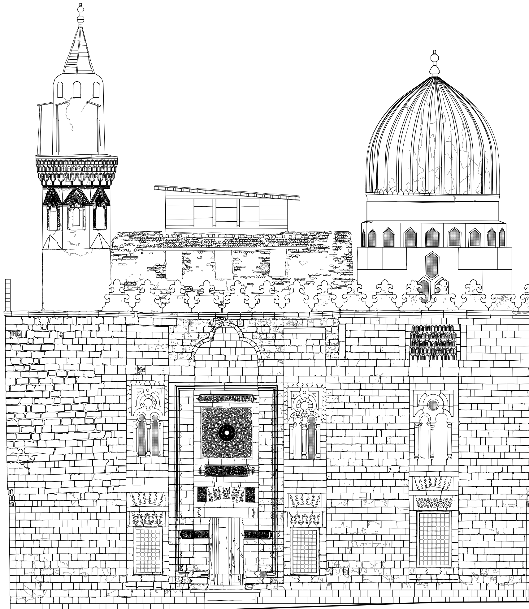
B 08 SOUTHERN ELEVATION
