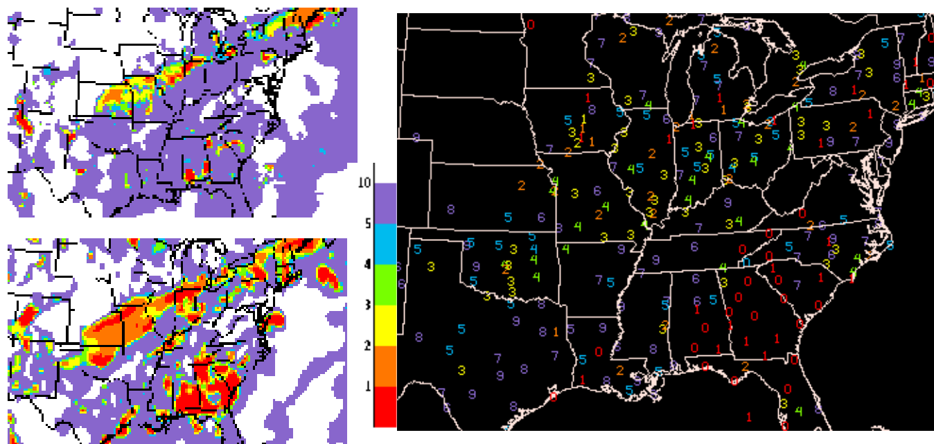
Figure 13. Visibility (mi) valid at 1200 UTC 30 January 2002. a) RUC40 00-h forecast, b) RUC20 0-h forecast, c) METAR observations.
