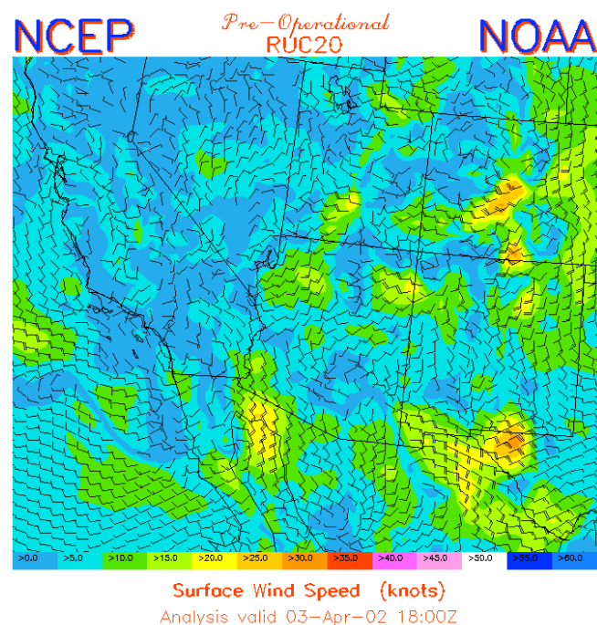
Figure 3. Verifying analysis of surface winds at 1800 UTC 3 April 2002 from RUC20 for a) 40km resolution plot and b) 20km resolution plot over Colorado.
