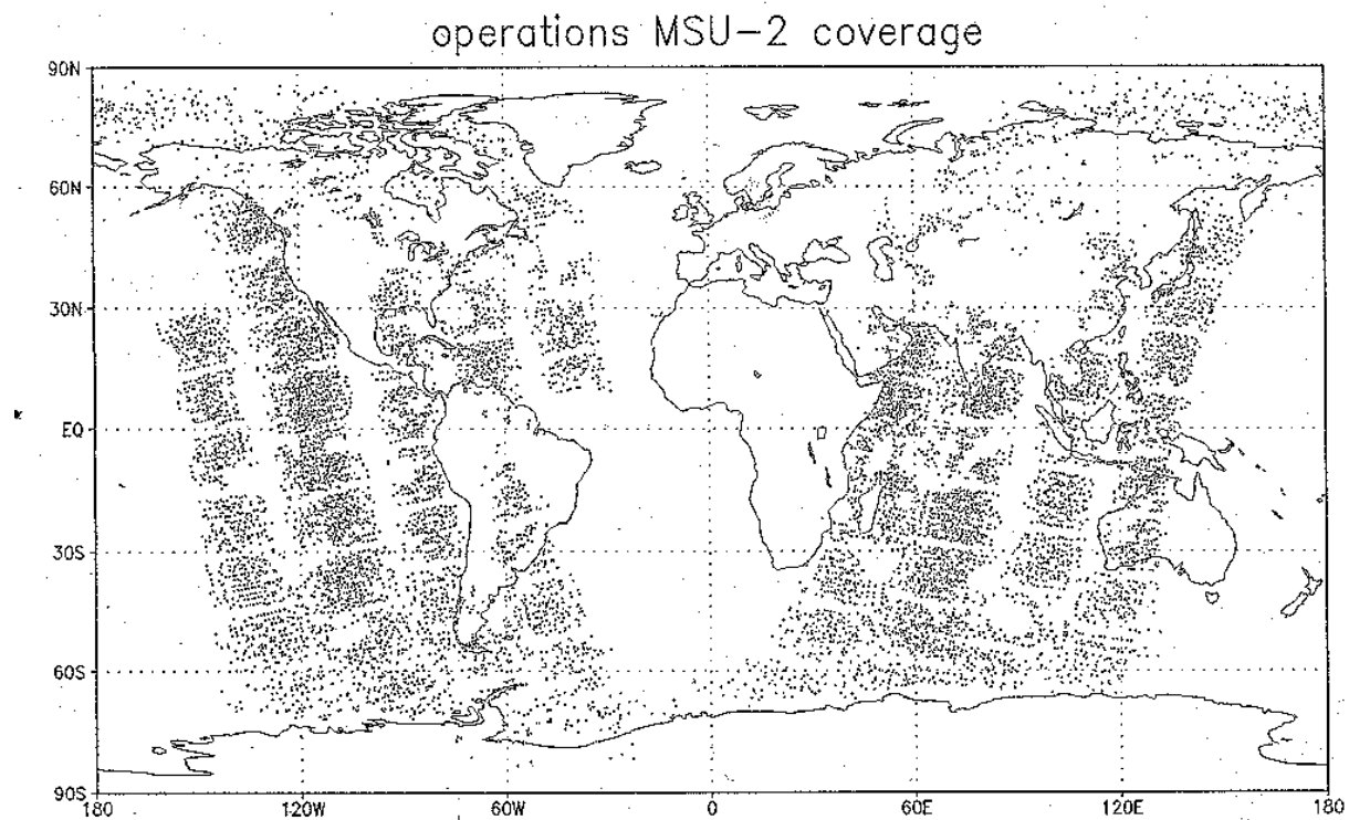
Fig. 5 MSU channel 2 data locations for 6-h period operationally available from NESDIS pre-processed TOVS radiances after quality control (top); same except level-1b data (bottom).
