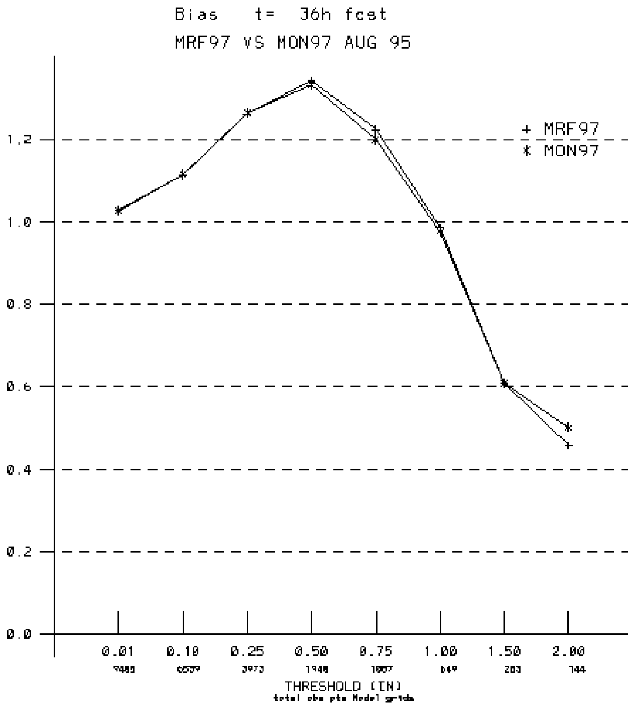
Fig. 12 As in Fig. 11, but for bias
