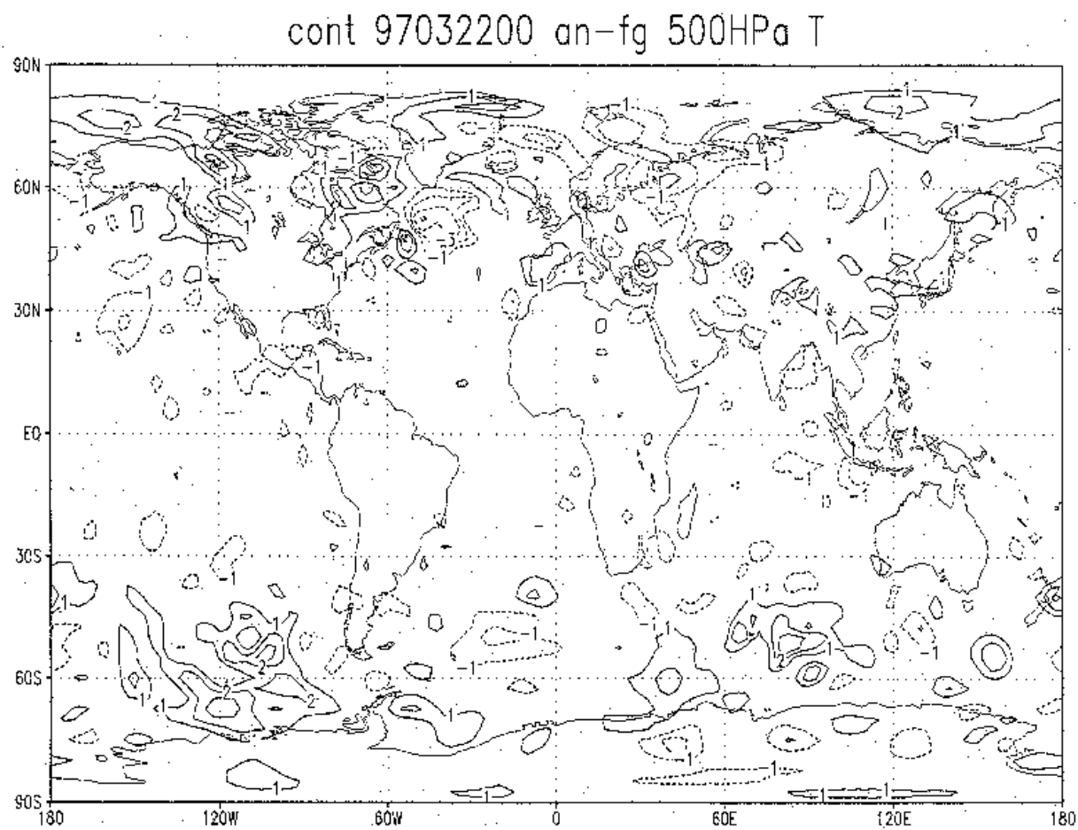
Fig. 6 Analysis minus background (6-h forecast) difference for 500 hPa temperature field using NESDIS pre-processed TOVS radiances, date of analysis 22 March 0000GMT (top); same except using level-1b data (bottom).
