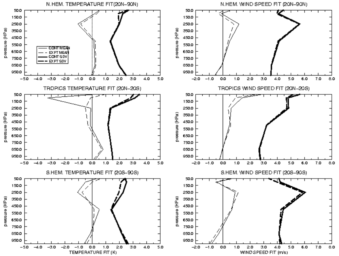
Fig. 8 Fits to data, i.e., observation minus background (6-h forecast) differences and standard deviations for assimilation using NESDIS pre-processed radiances (solid) and level-1b radiances (dashed) averaged over various regions (rows) for temperatures and winds. The biases are the thin pair of curves in each graph.
