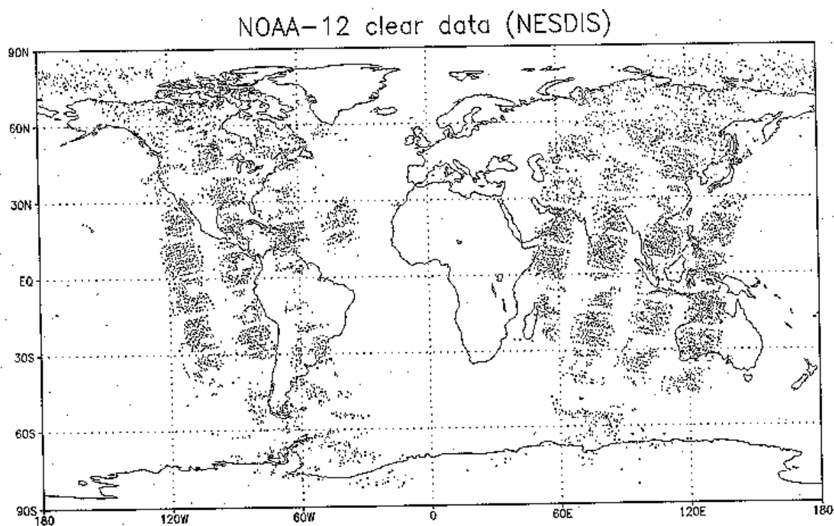
Fig. 4 HIRS channel 10 locations for 6-h period operationally available from NESDIS pre-processed TOVS radiances (top); same, except for level-1b data (bottom).
