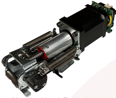
Motorized Latch Retraction
