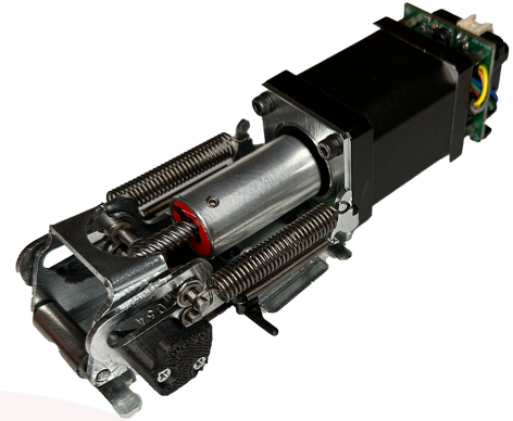
Motorized Latch Retraction
