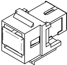
ASSEMBLED VIEW SCALE 1.5:1
