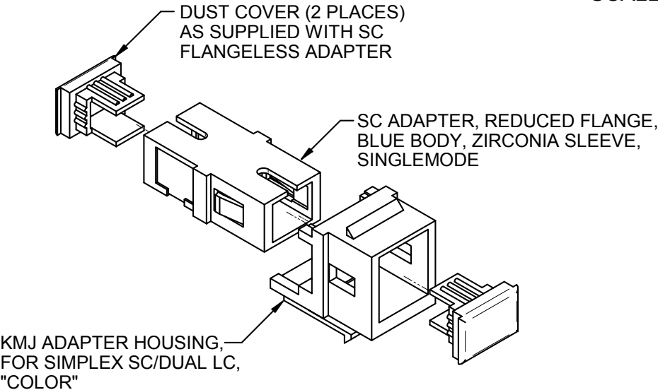
EXPLODED VIEW SCALE 1.5:1
