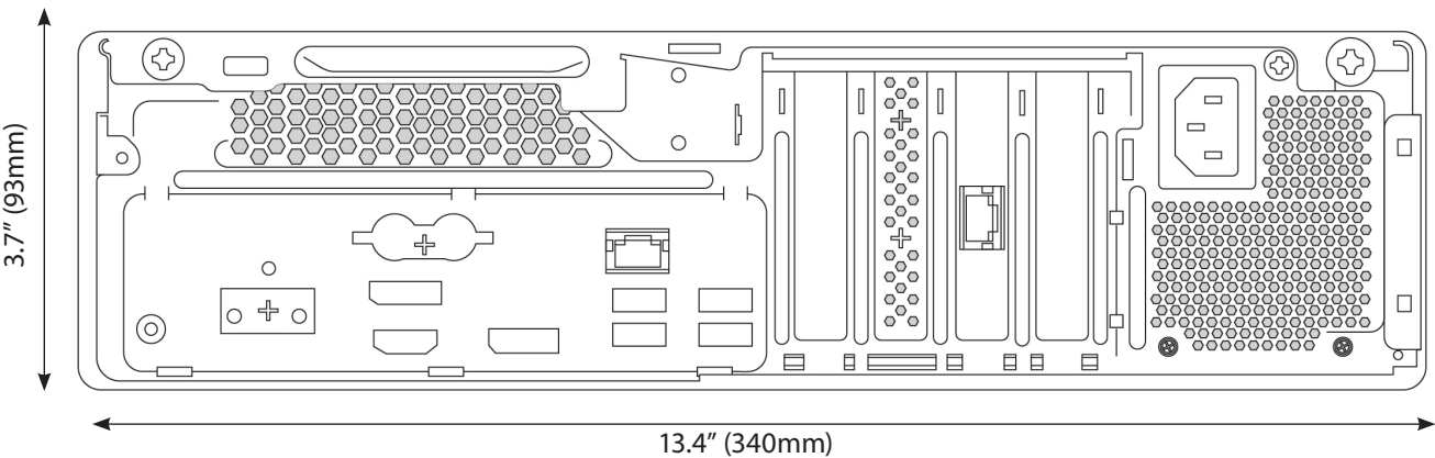
Rear View
