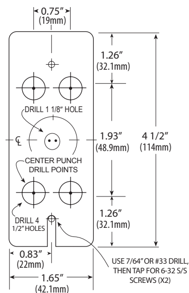
CUTTING TEMPLATE
