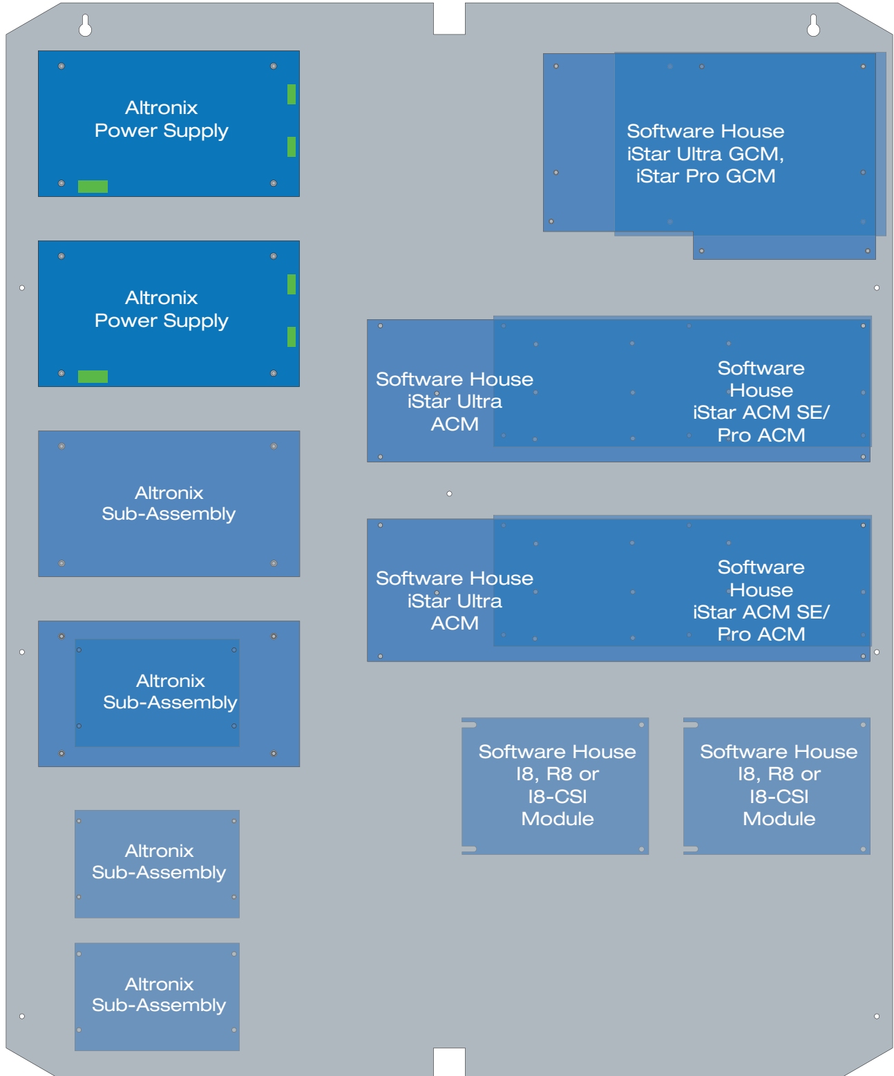
Trove3SH3 Interior Backplane - Optional Mounting Configurations
