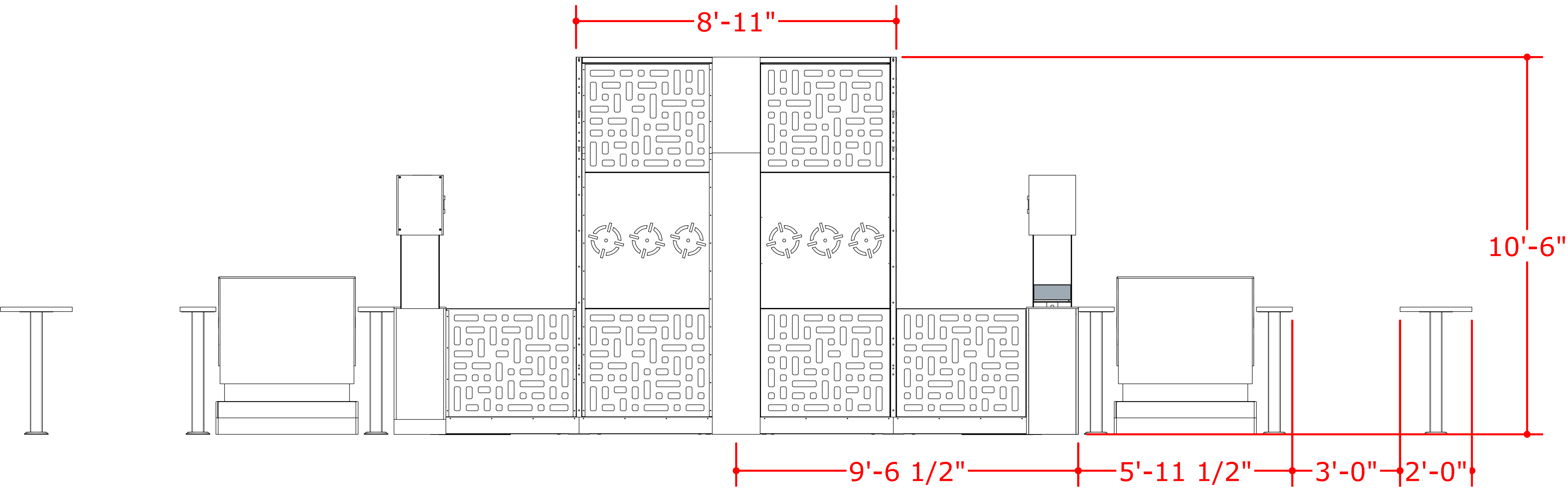
2-LANES - BACK TO BACK - SIDE VIEW
