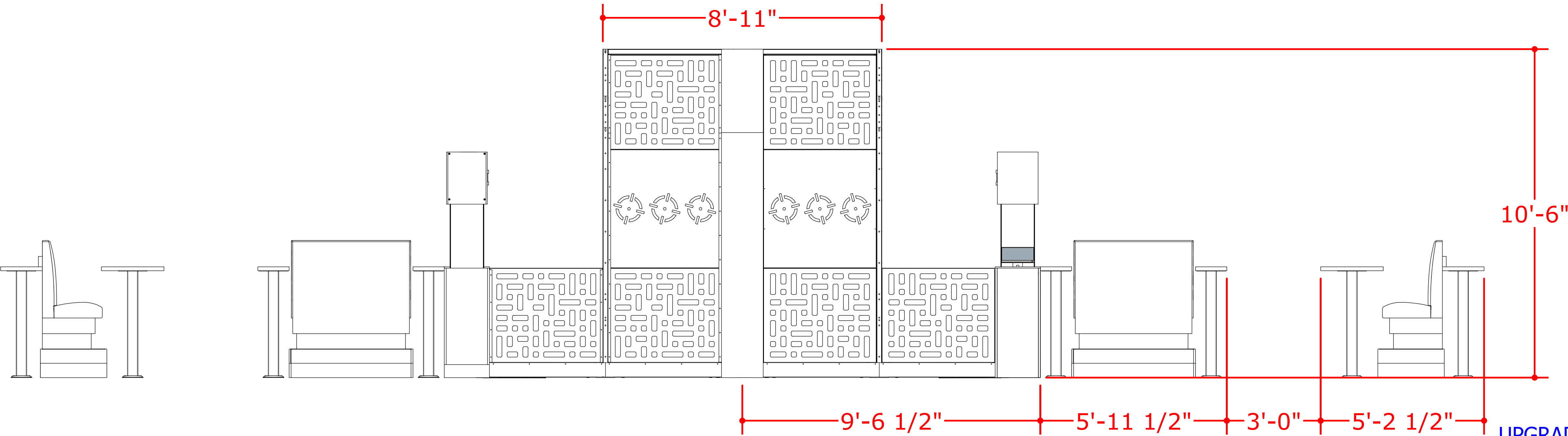
2-LANES - BACK TO BACK - SIDE VIEW
