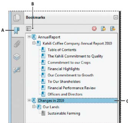
Bookmarks panel
