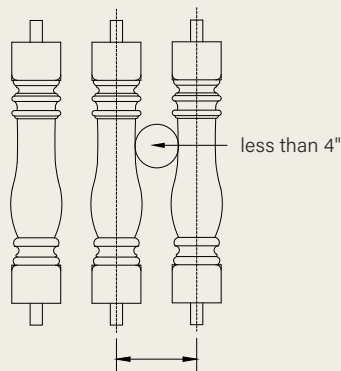
Center-to-Center Distance
