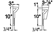
Standard w/ Keystone K6M
