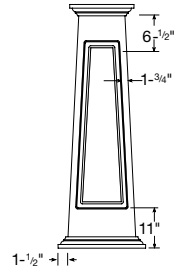
Route is 1-3/8" wide by 3/8" deep.
