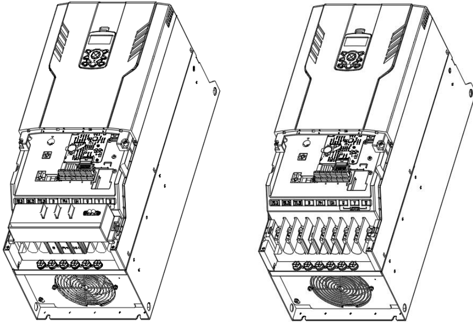
Figure 7. Remove Power Cover and CABLE Guide
