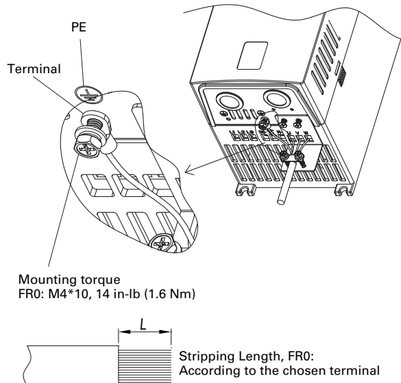
Figure 30. FR0 grounding
