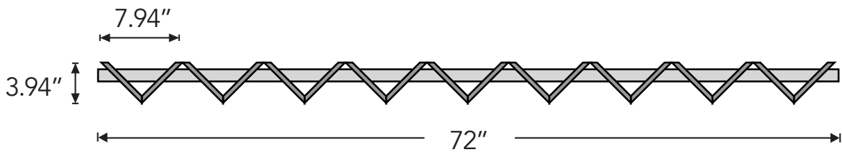
Side View
