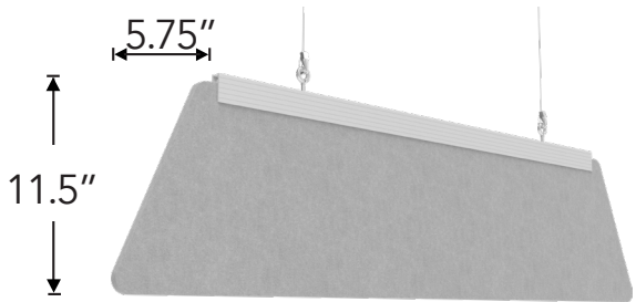
Capsule Baffle
