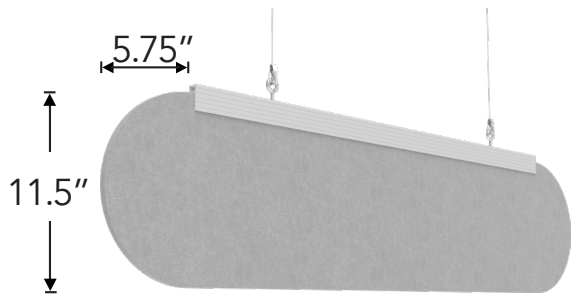
Capsule Baffle
