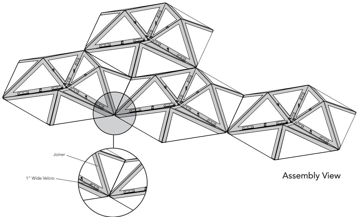
Joiner Detail
