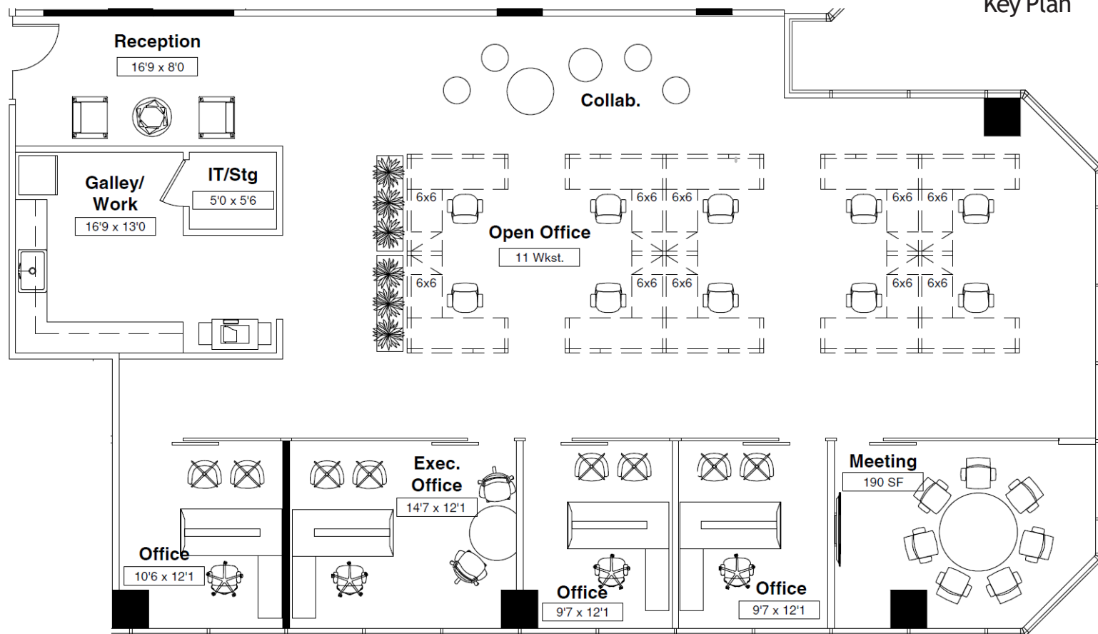
Key Plan
