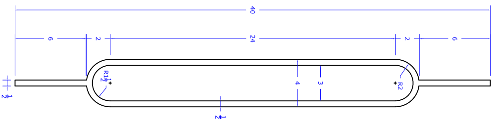
Detail 01: Front View Scale: 1\frac{1}{2}'' = 1'-0''
