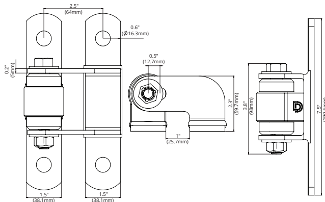
CI3720 Drawing
