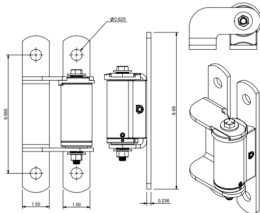
CI3860FM combines the CI3835FM + CI3720 CI3835FM Drawing
