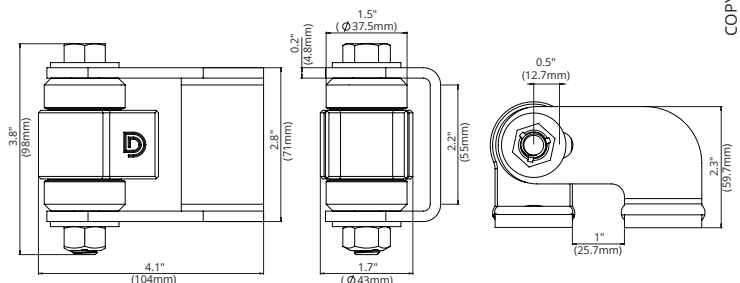
CI3050 Drawing
