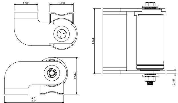
CI3850FM combines the CI3825FM + CI3050 CI3825FM Drawing
