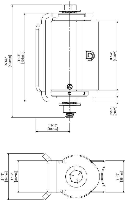
CI3825R Drawing
