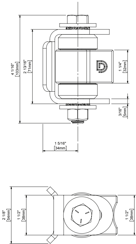
CI3000R Drawing
