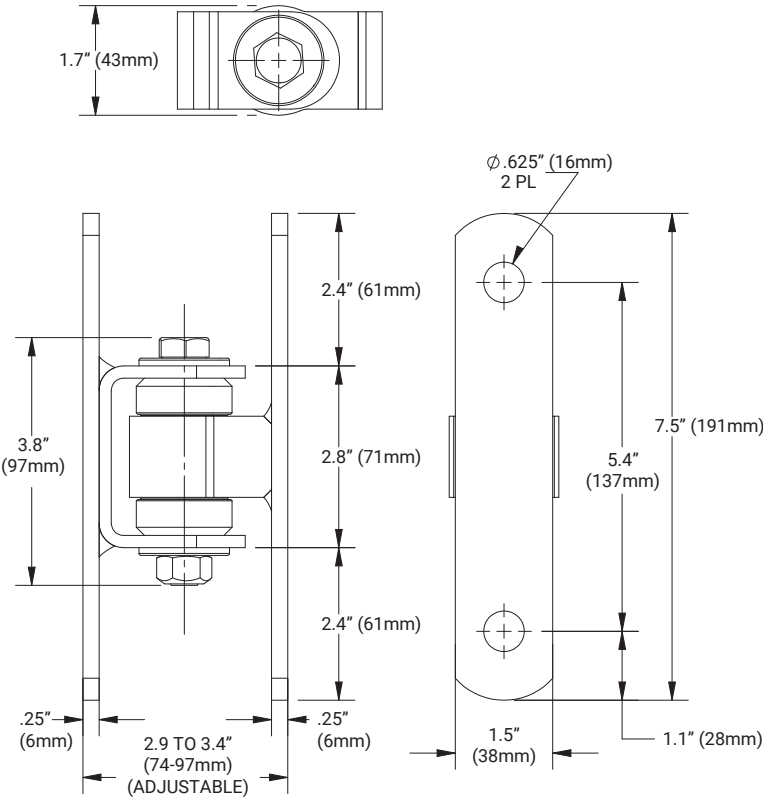
CI3700 Drawing
