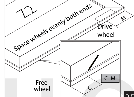
Free wheel backset
