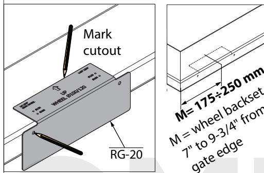
Secondary drive wheel backset
