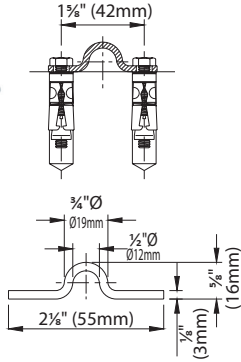
291 Alignment pin for 289G track
