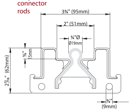
287FP-G-19.68FT 287FP-G-9.84FT Galvanized, recessed guide so track is mounted at floor level Track and connector rods sold separately.
