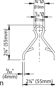
297 Alignment pin for 287G track
