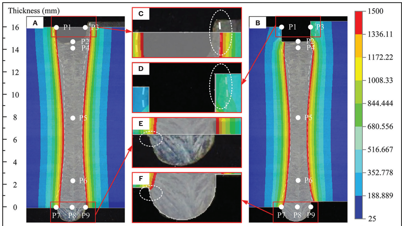
Fig. 6 — Comparison of the experimentally measured and numerically predicted weld bead cross sections of: A — M1; B — M3. C–F is the magnification of the weld bead cross section top and bottom of M1 and M3.
