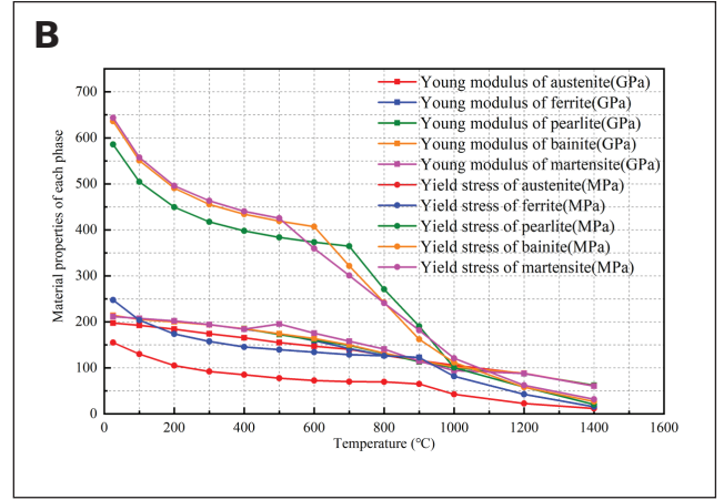
Fig. 5 – Temperature-based material properties of: A – EH40 steel; B – each phase.
