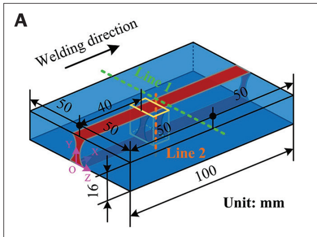
Fig. 2 — A — The size of the EH40 butt joint, the test position (Line 1) of residual stress; B — Line A, Line B, and Line C of hardness.
