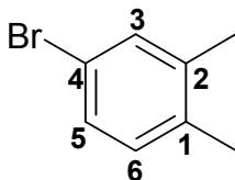
4-bromo-1,2-dimethylbenzene
