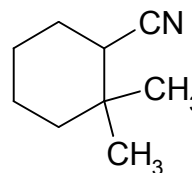
2,2-dimethylcyclohexanecarbonitrile
