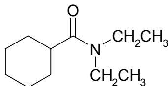
N,N-diethylcyclohexanecarboxamide
