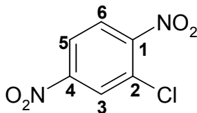
2-chloro-1,4-dinitrobenzene
