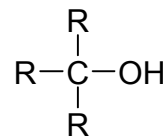
tert ROH
