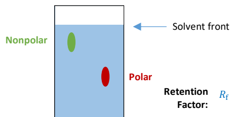
Thin-Layer Chromatography
