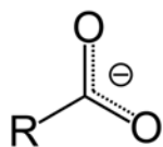
Carboxylate Ion
