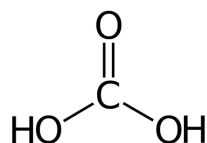
Carbonic Acid
