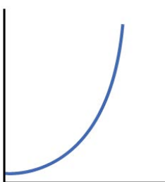
Exponential Relationship
