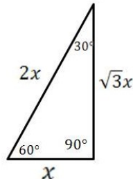
30-60-90 triangle
