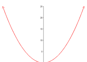
Quadratic Relationship
