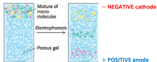
Gel electrophoresis
