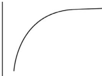
Logarithmic Relationship
