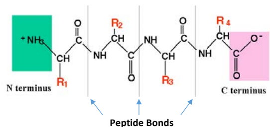
Polypeptide Structure
