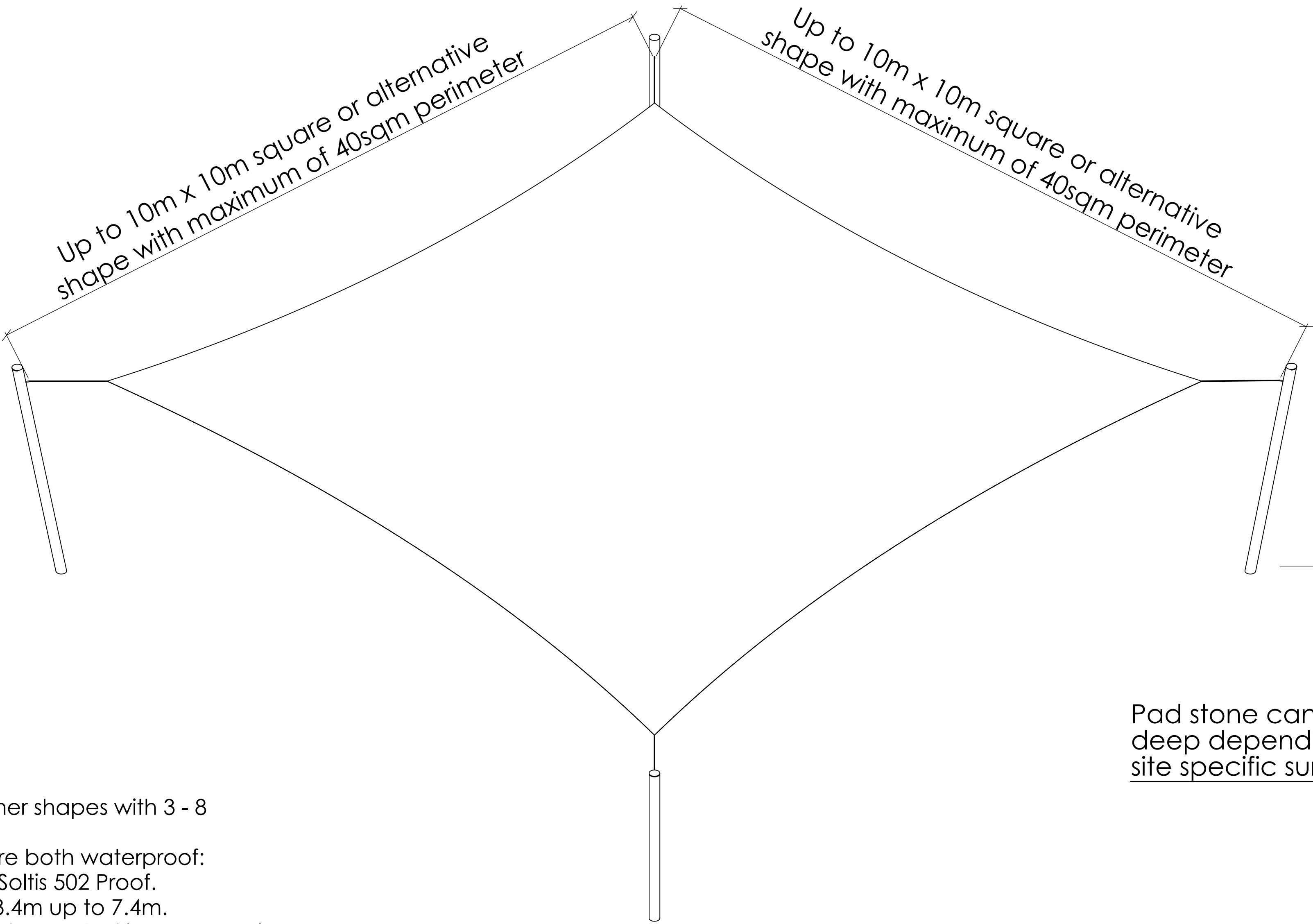
Front view
