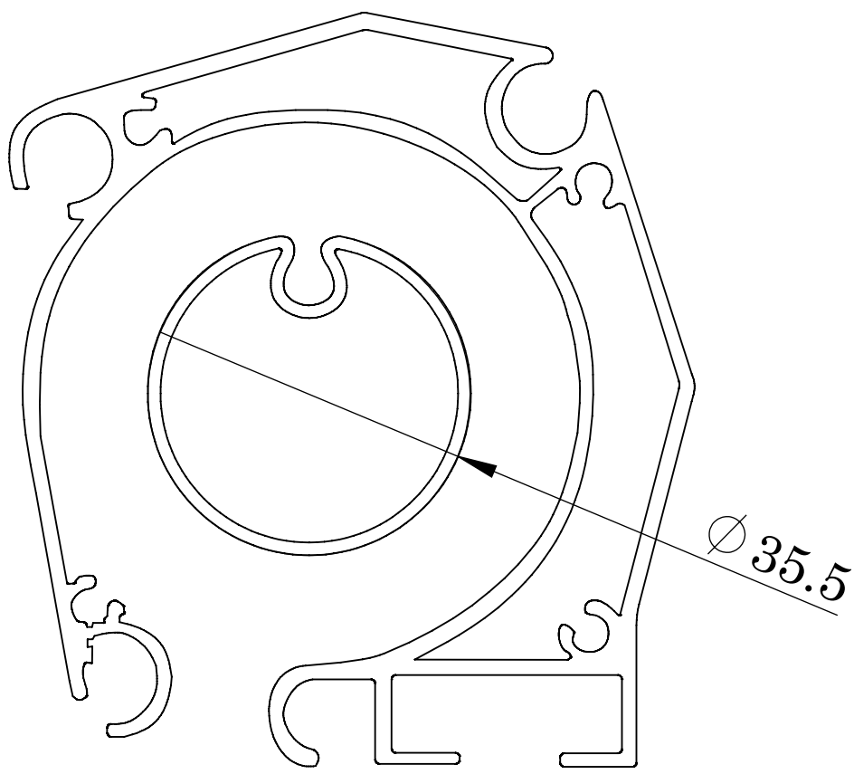
Front bar with crank for Vario Volant system
