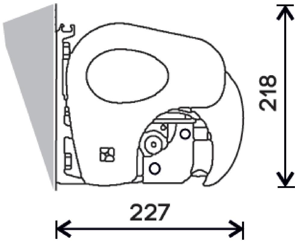
WALL INSTALLATION
