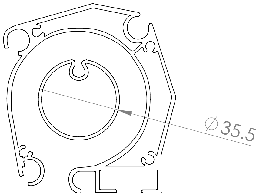
Front bar with crank for Vario Volant system
