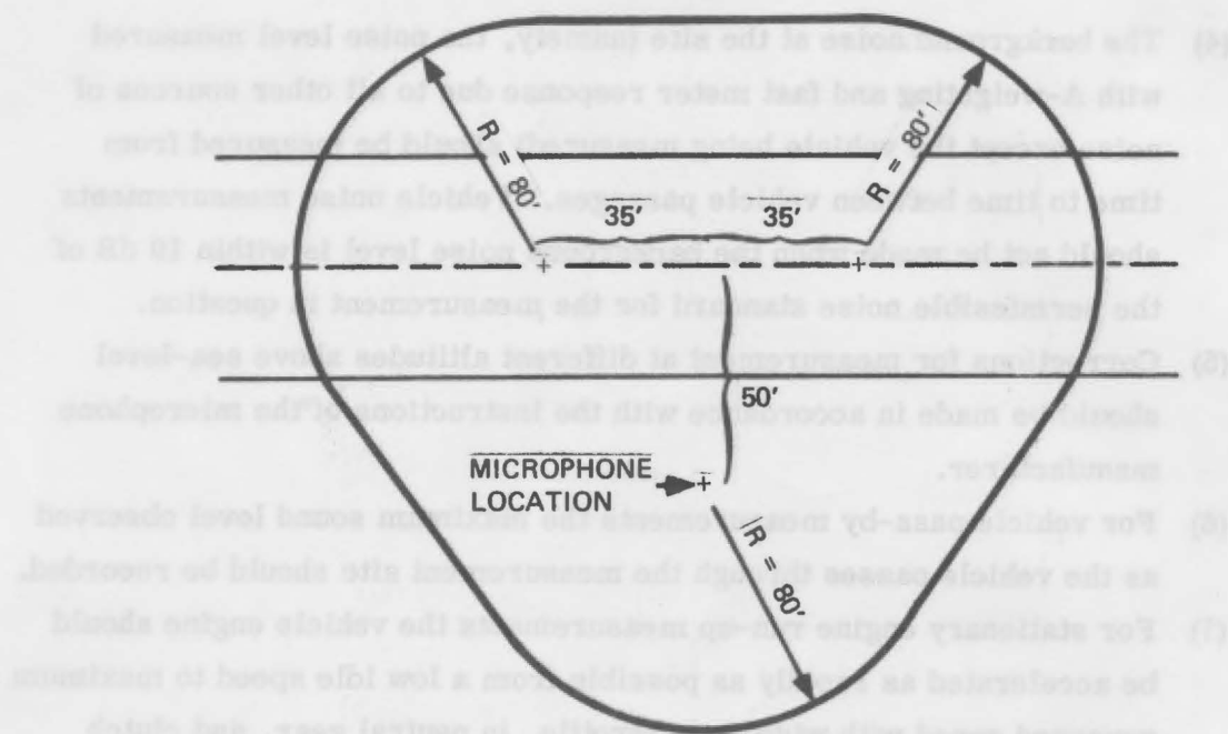
Figure A-1. Test site clearance requirements for pass-by test.
