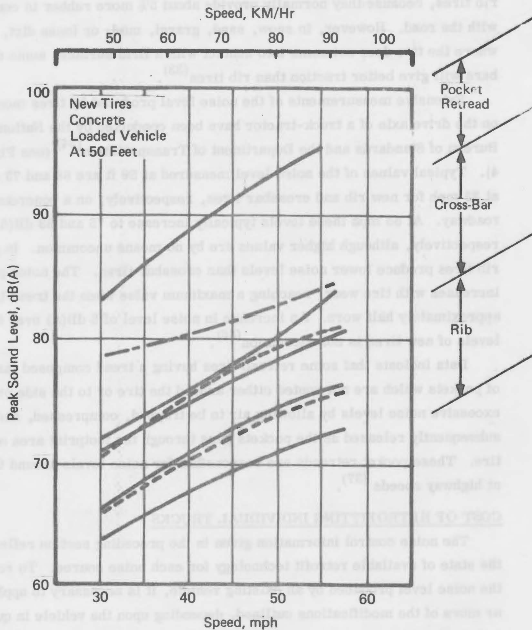
Figure 4. Peak A-Weighted Sound Level, as Measured at 50 Feet, Versus Speed for a Loaded Single-Chassis Vehicle Running on a Concrete Surface. Various Types of New Tires are Represented on the Graph. These Were Mounted on the Drive Axle (35)
