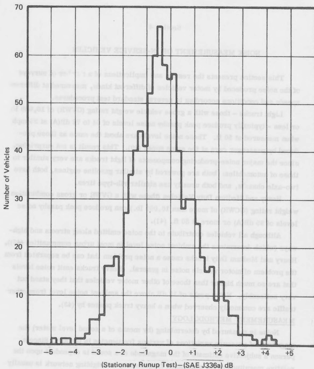
Figure 9. (Stationary Run-up Test) - (SAE J336a), dB
