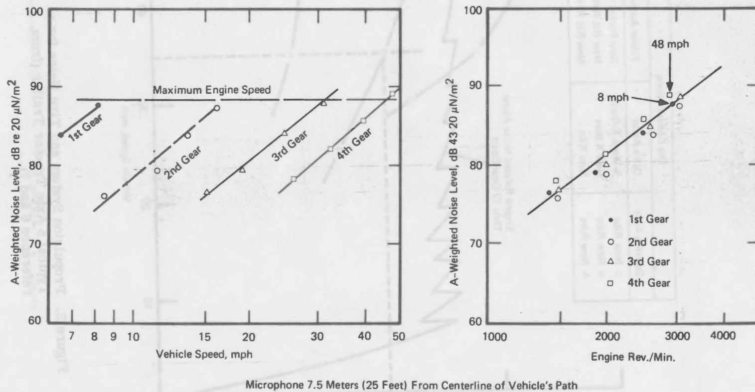
Figure 1. Propulsion System Noise Versus Vehicle Speed and Engine Speed
