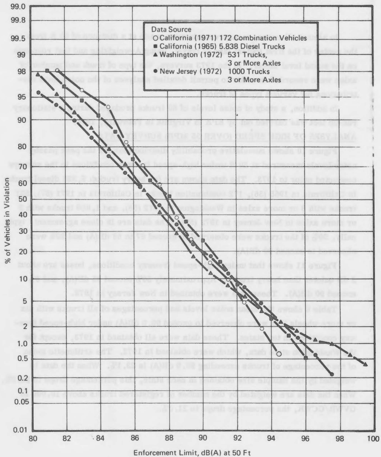
Figure 10. Enforcement Limit, dB(A) At 50 Ft
