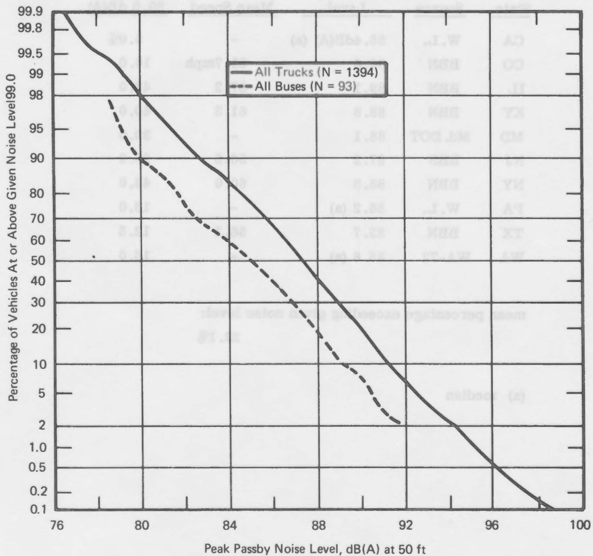
Figure 11. Cumulative Distribution Of Peak Passby Noise Levels For All Trucks And All Buses At Speeds Over 35 MPH
