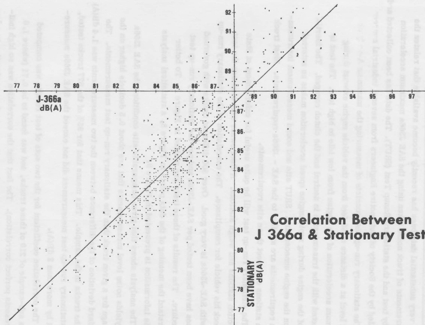
Figure 8. Plot of Test Results According to SRUT and SAE J366a for 877 Trucks.
