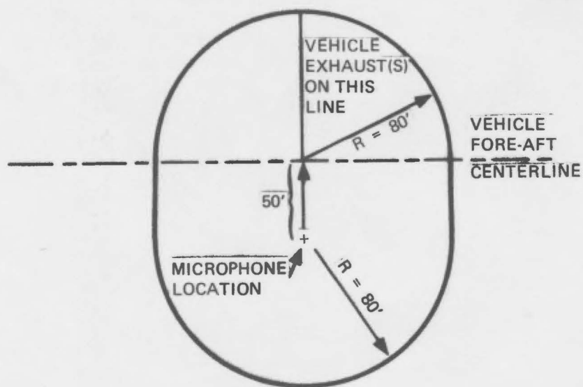
Figure A-2. Test site clearance requirements for stationary run-up test.
