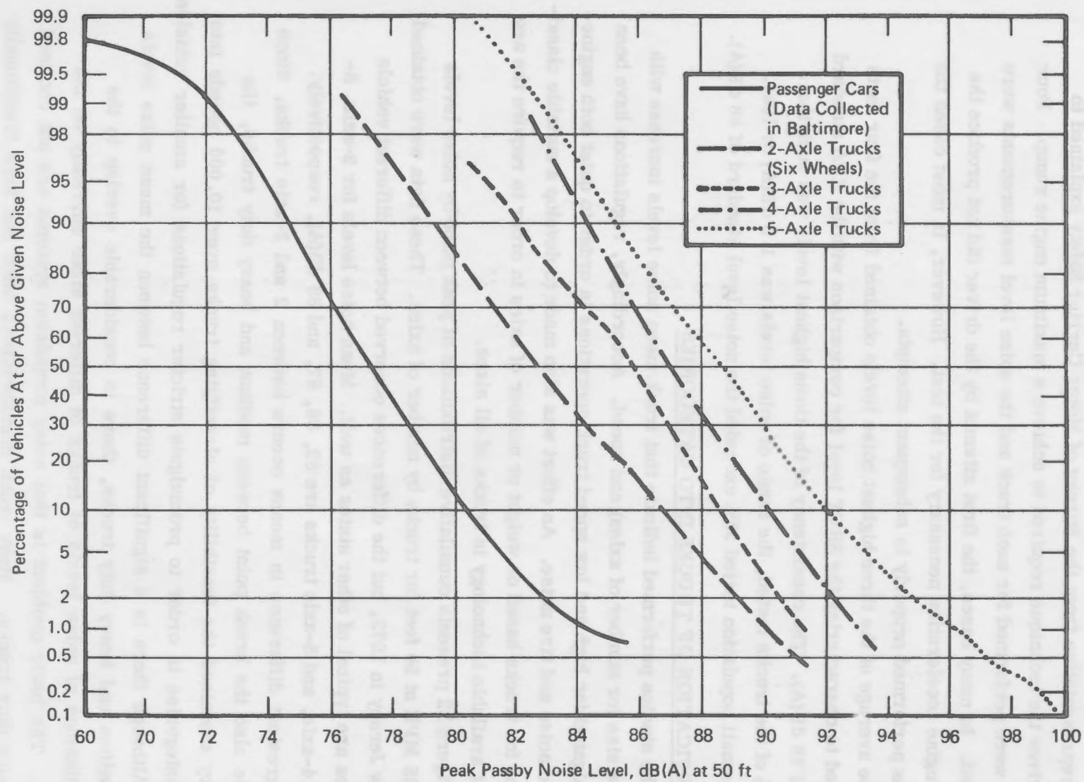
Figure 12. Cumulative Distribution of Peak Passby Noise Levels for Various Classes of Trucks at Speeds Over 35 MPH.
