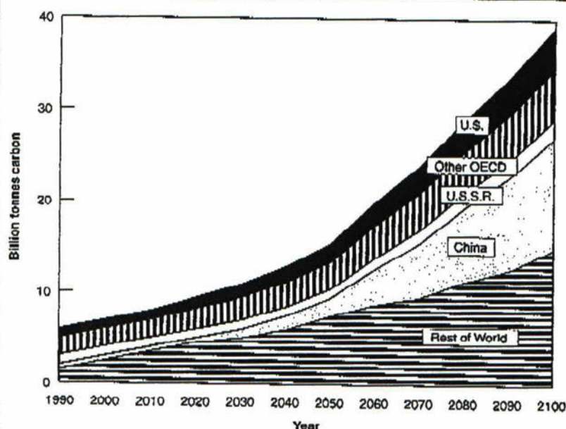
Figure 2 Relative Carbon Contributions of Different Regions to Global Carbon Emissions
